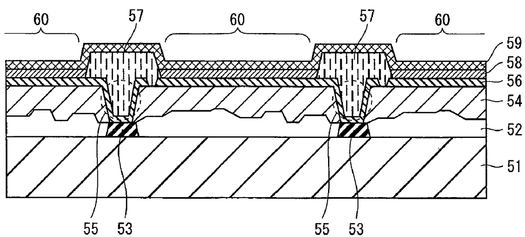
FIG. 12 Prior art
